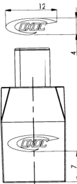
GA02ADC001AB0 With logo (Print Color=Silver)
