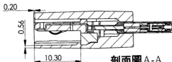
GA02ADC001AB0 With logo (Print Color=Silver)
